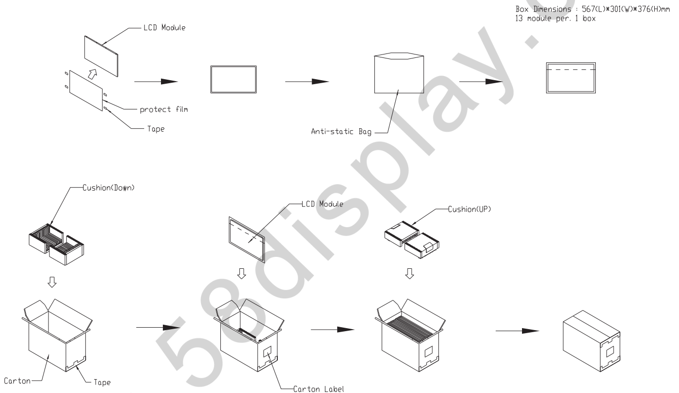
Figure. 8-1 Packing method
