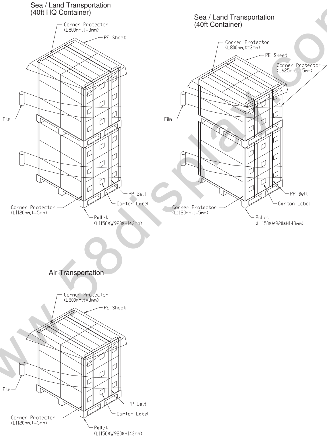
Figure. 8-2 Packing method
